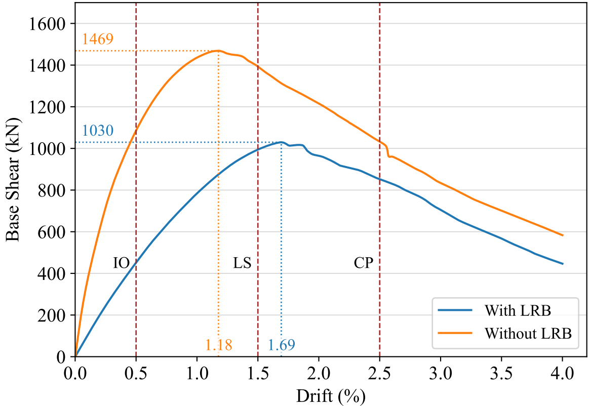
Pushover Curves for 750kL Tank
